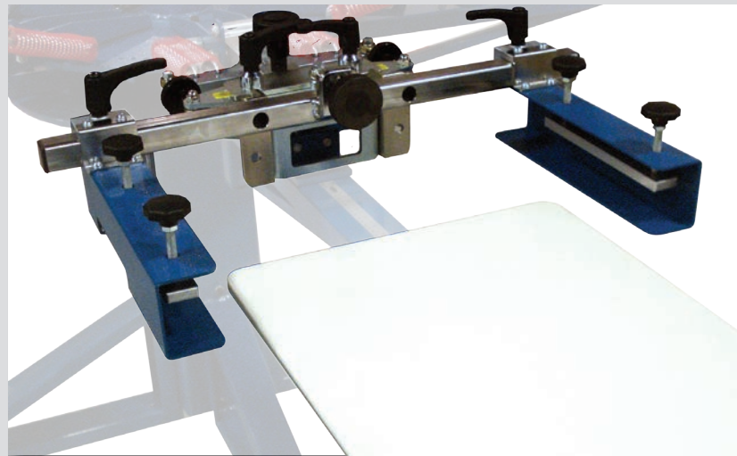
FULLY-ADJUSTABLE SIDE CLAMPS (OPTIONAL)
